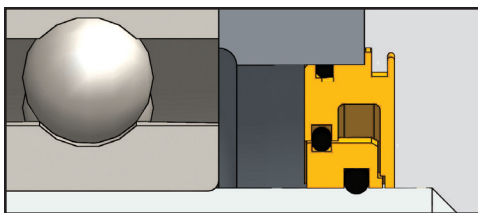
mini66 – 0.375" Overall Length
